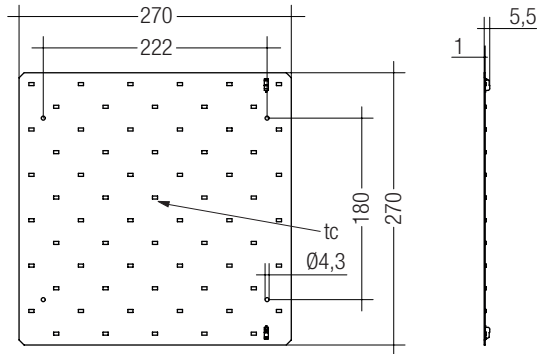
QLE-G3-270
