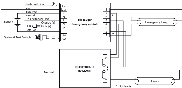
Twin series switch start circuit with high frequency electronic ballast
